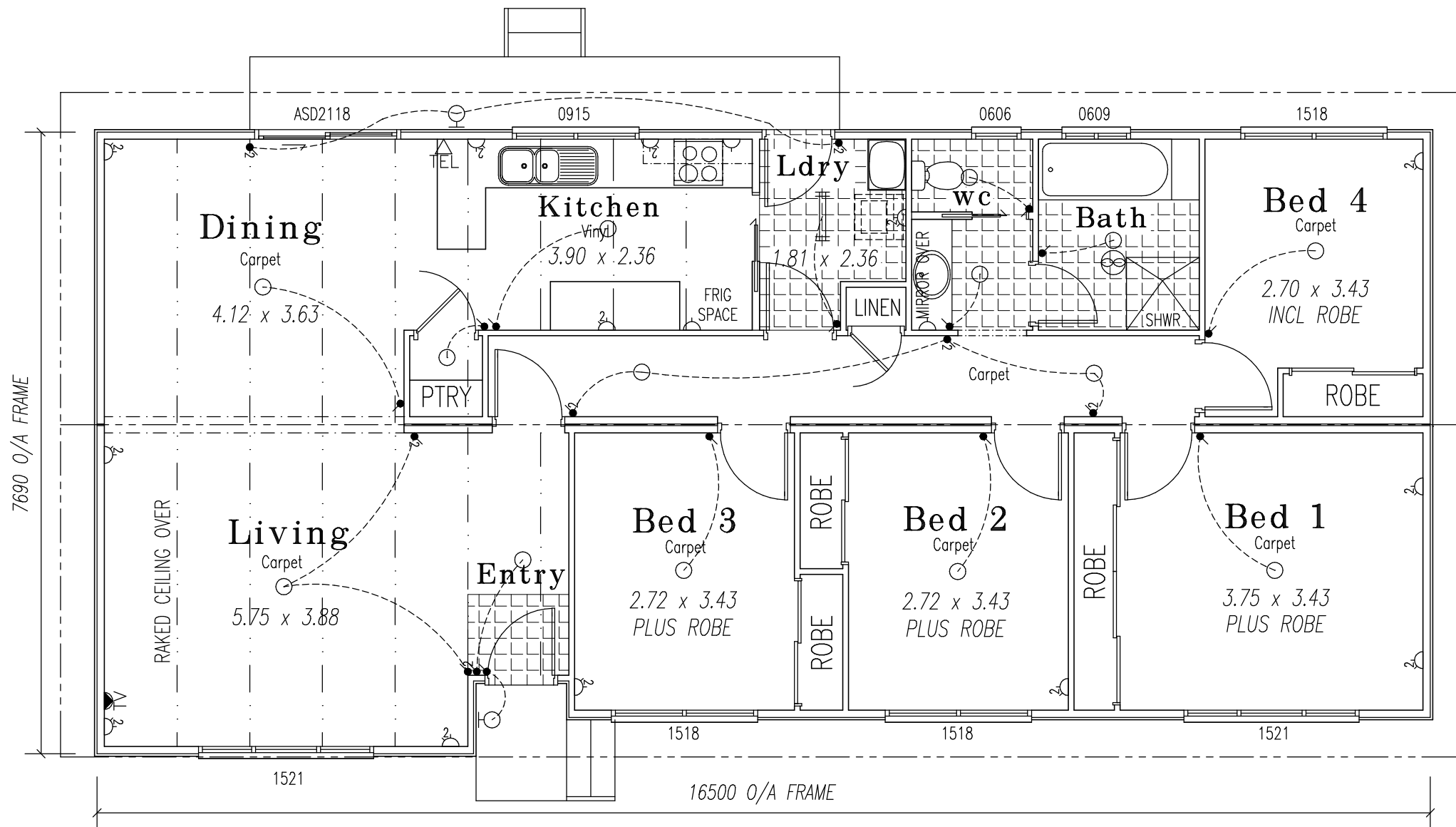
FLOOR PLAN
