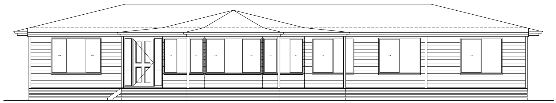
FRONT ELEVATION
