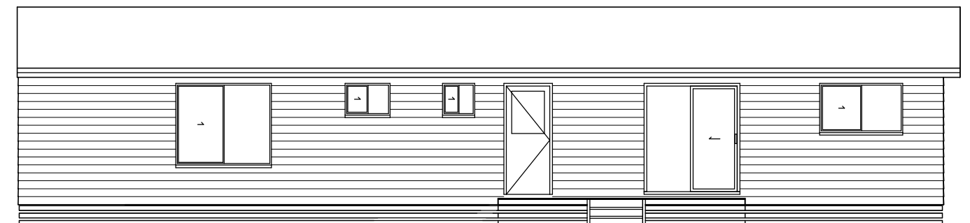
REAR ELEVATION
