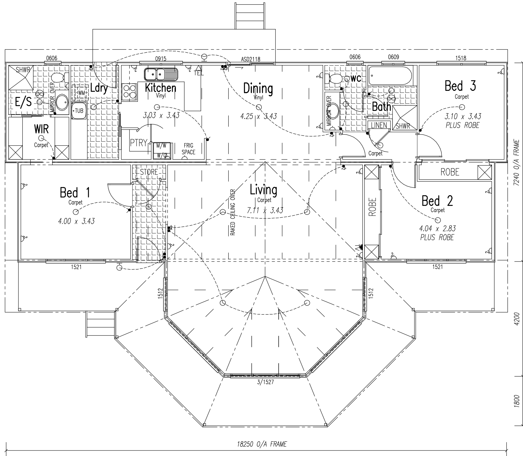
FLOOR PLAN
