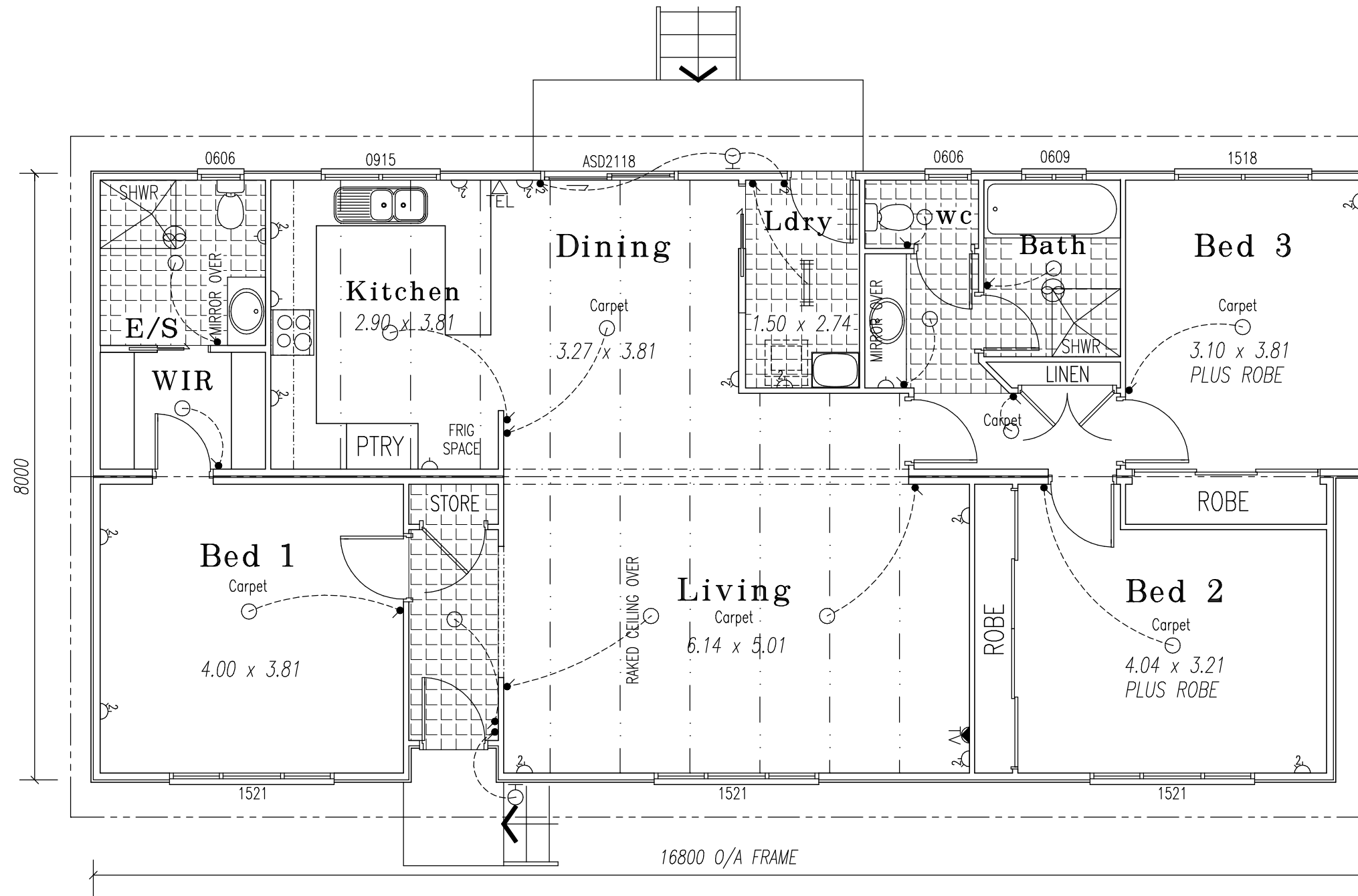
FLOOR PLAN
