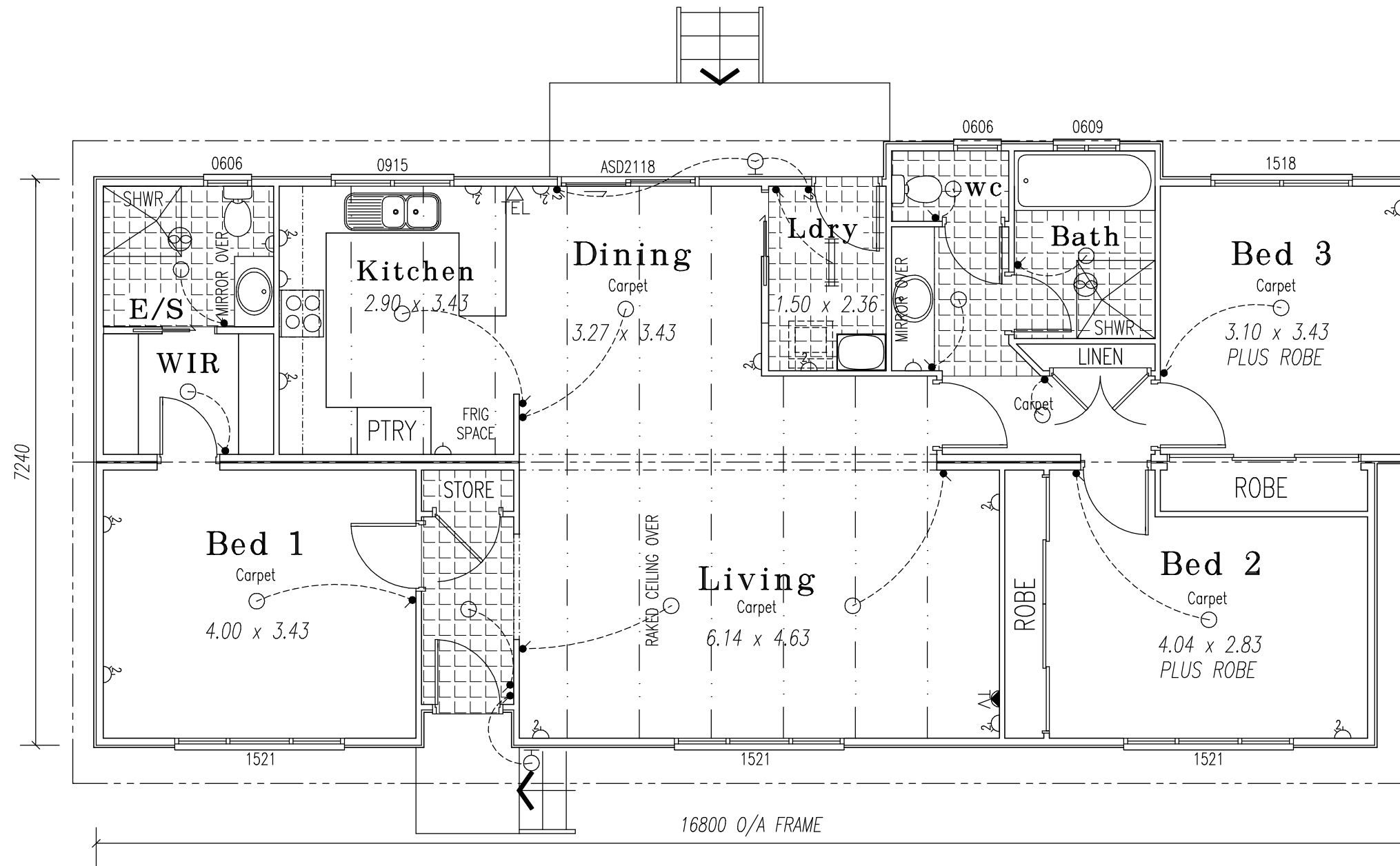
FLOOR PLAN
