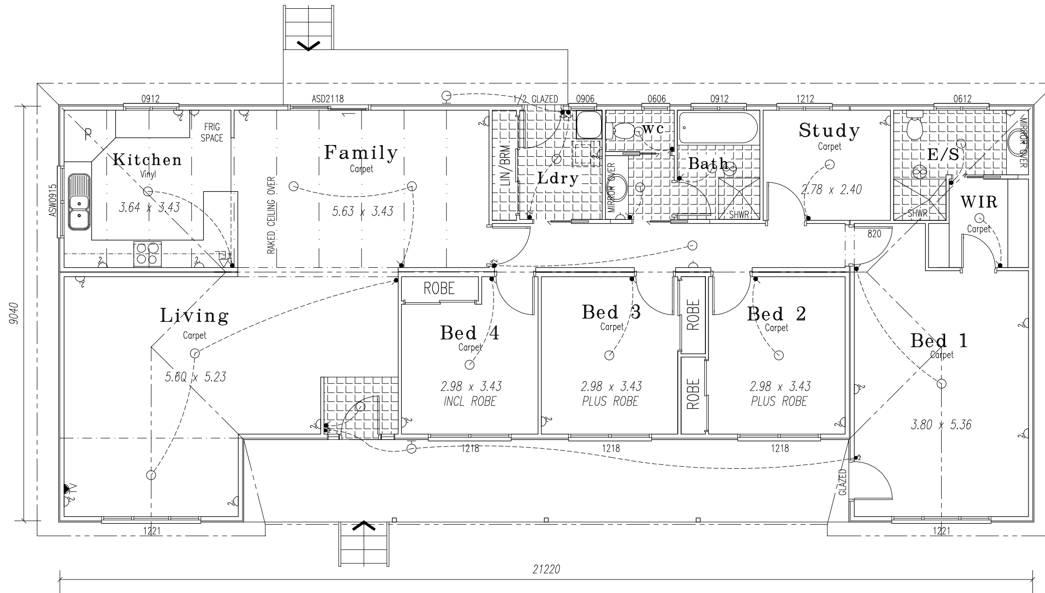
FLOOR PLAN
