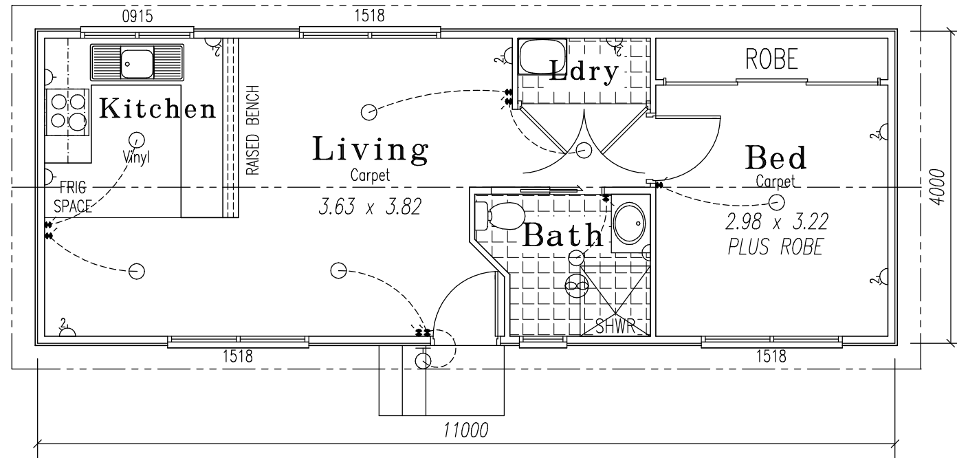
FLOOR PLAN
